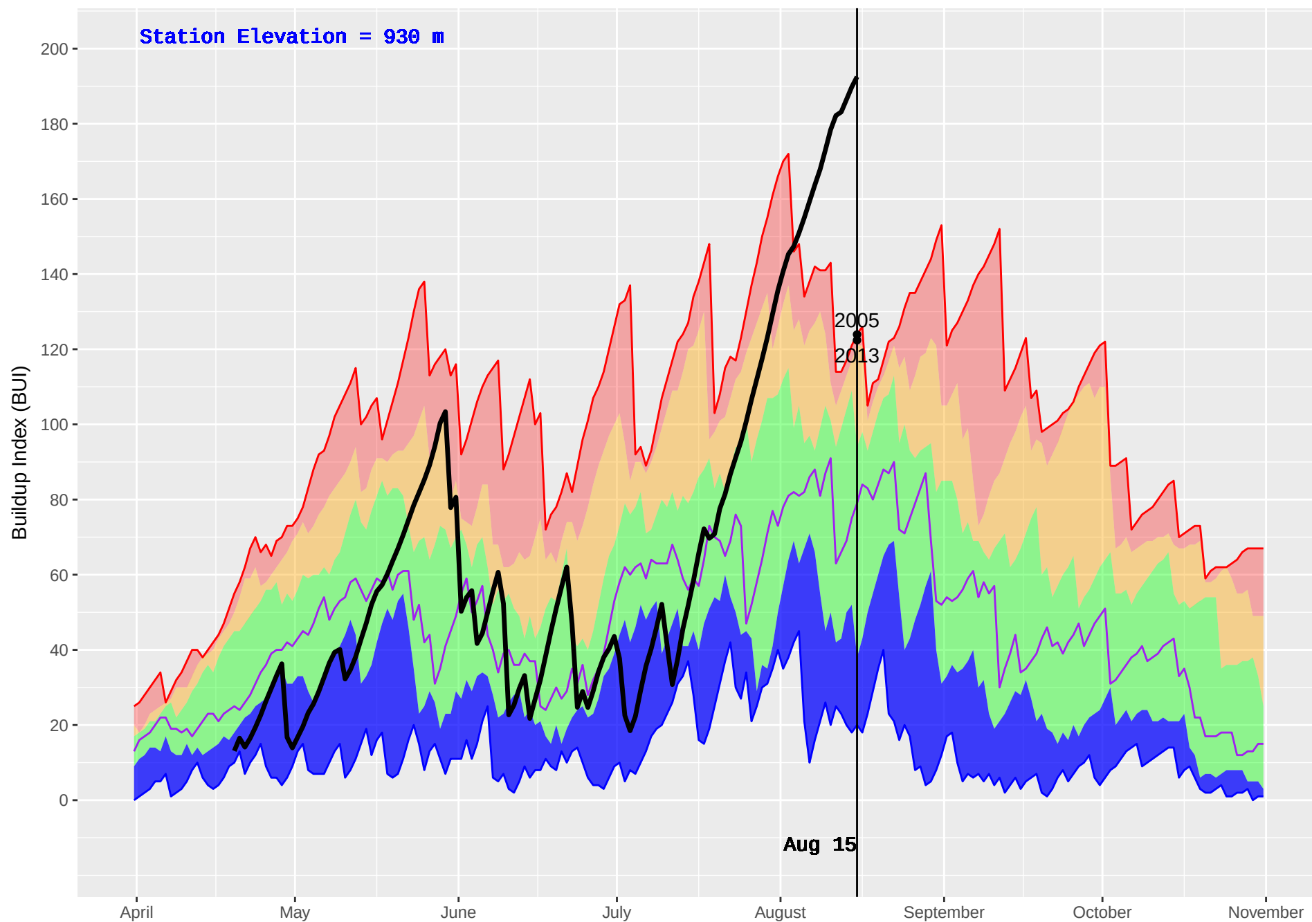
BRISCO (865) : Historical (2004–2016) and Current (2018) Daily Buildup Index (BUI)
