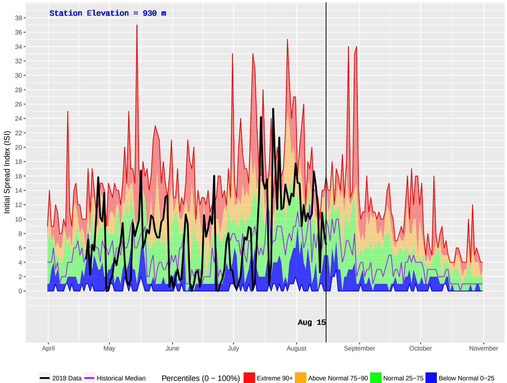
BRISCO (865) : Historical (2004–2016) and Current (2018) Daily Initial Spread Index (ISI)
