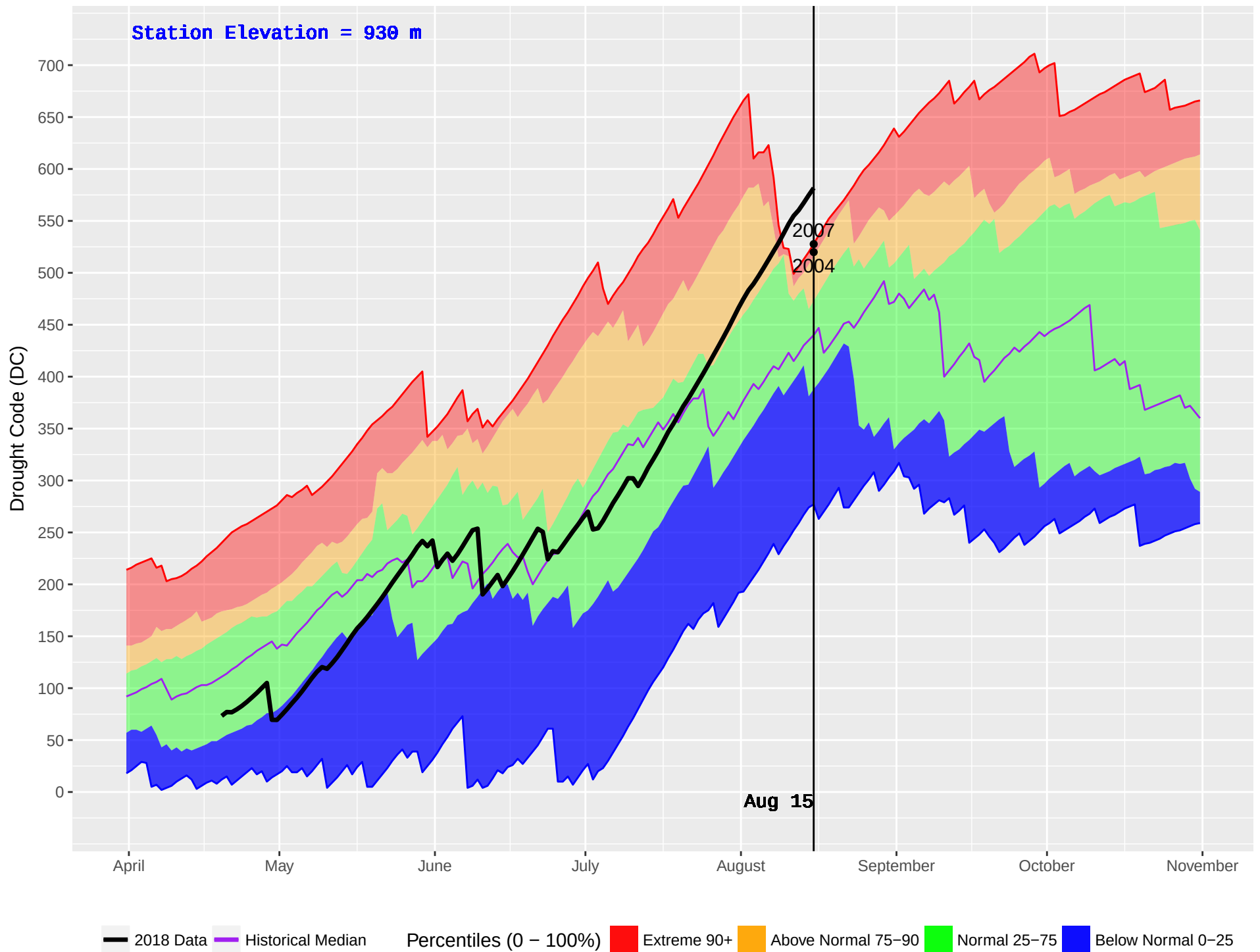
BRISCO (865) : Historical (2004–2016) and Current (2018) Daily Drought Code (DC)
