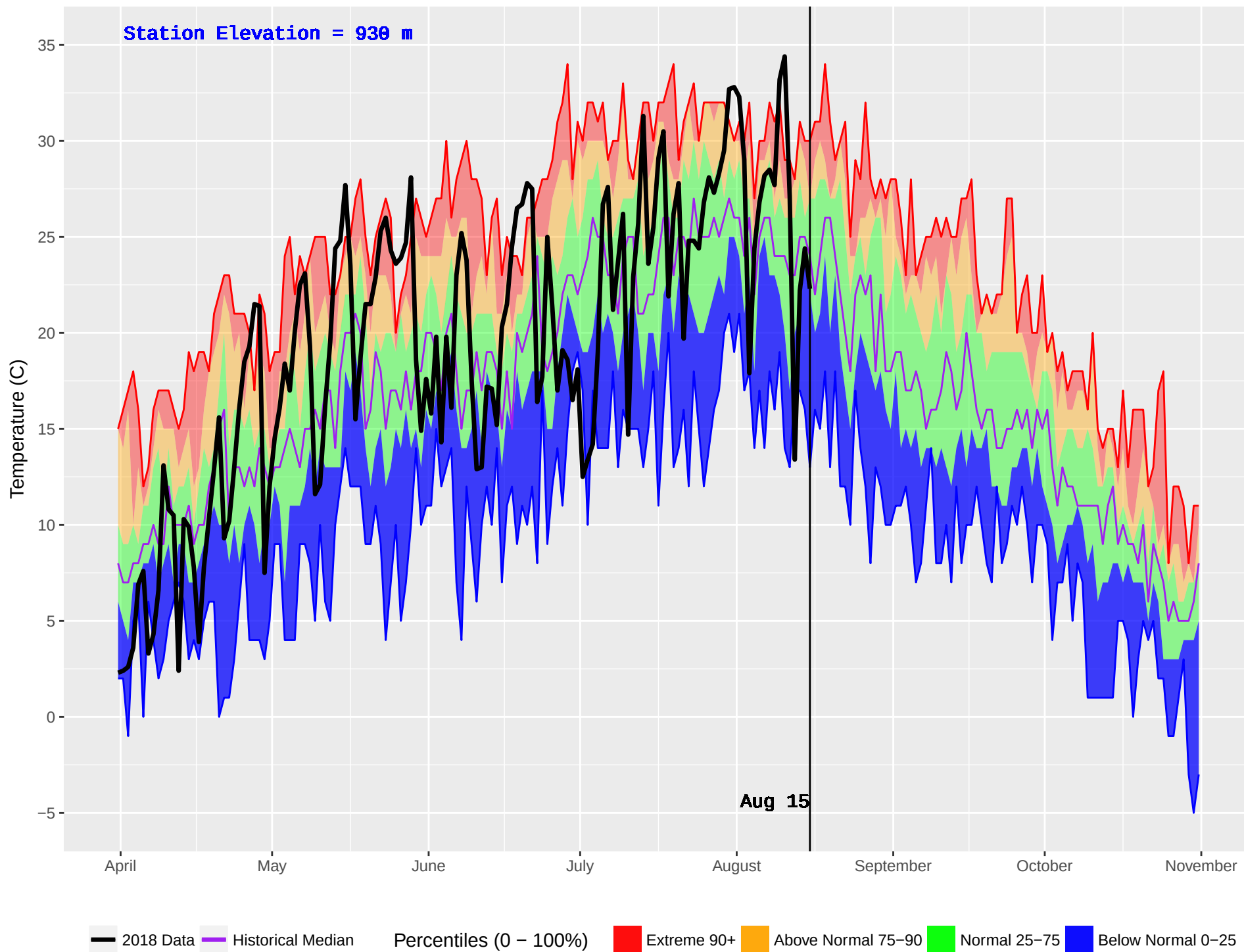
BRISCO (865) : Historical (2004–2016) and Current (2018) Daily Temperature
