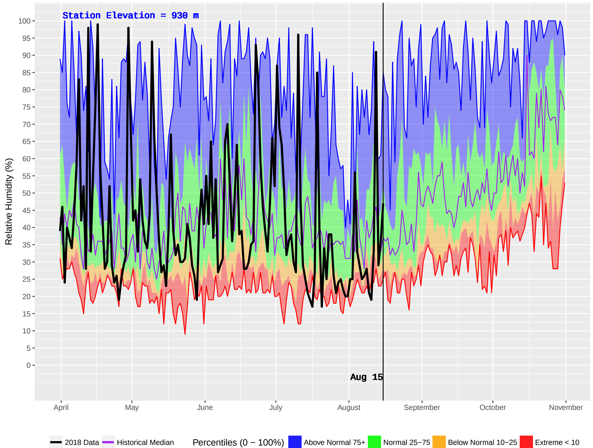
BRISCO (865) : Historical (2004–2016) and Current (2018) Daily Relative Humidity
